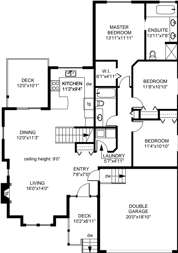
MAIN FLOOR 1574 SQ.FT
