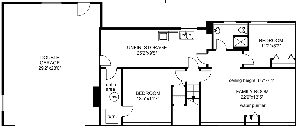
LOWER FLOOR 1180 SQ.FT
